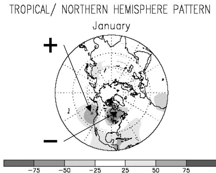
Figure 12. Phases of TNH pattern (modified by CPC, 2001).
